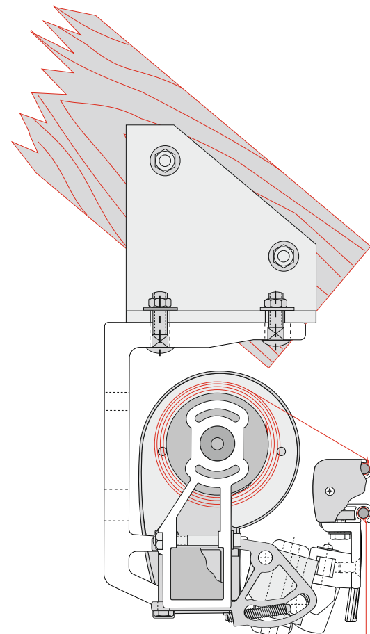
Dachsparrenmontage Rafter mounting
