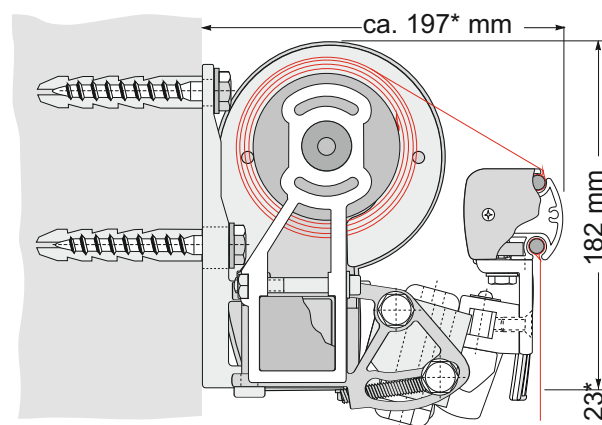
Wandmontage Wall mounting
