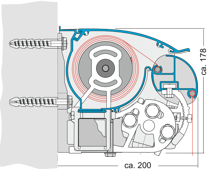
Wandmontage Wall mounting
