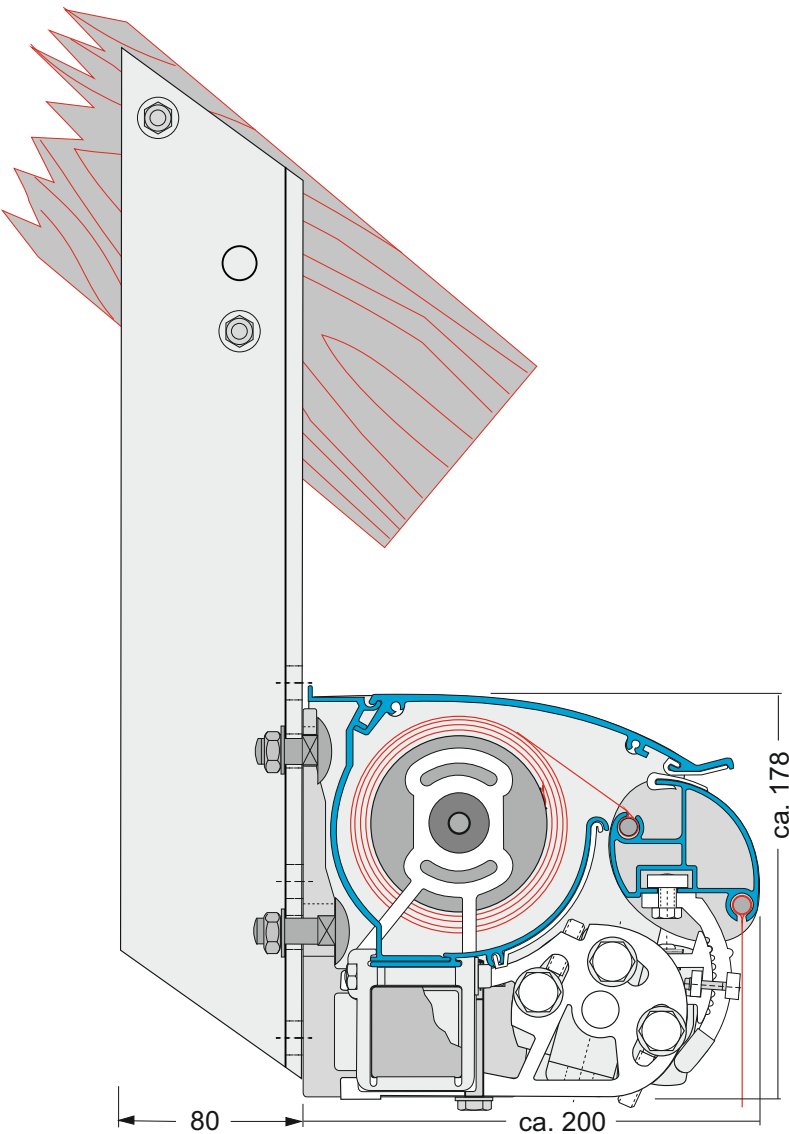
Dachsparrenmontage Rafter mounting
