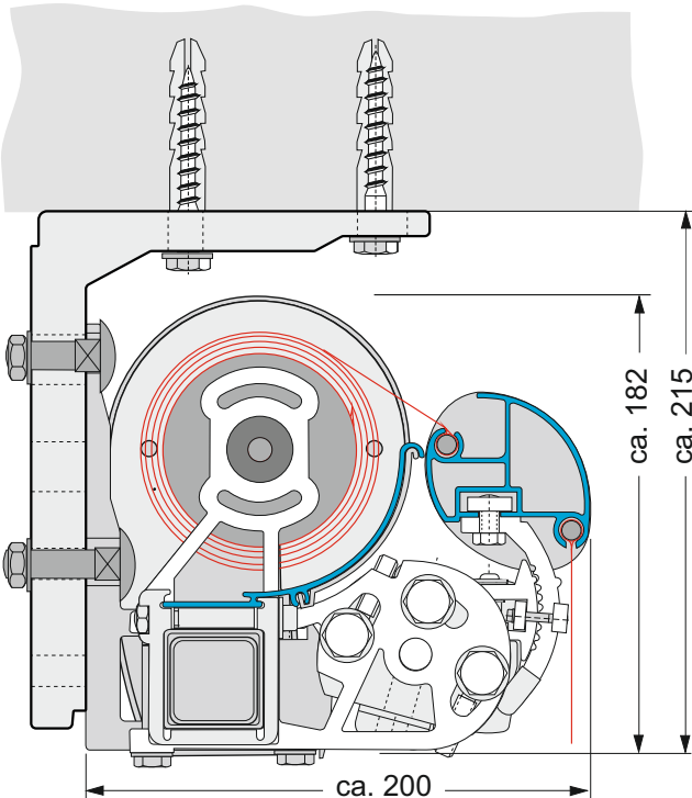
Deckenmontage Ceiling mounting
