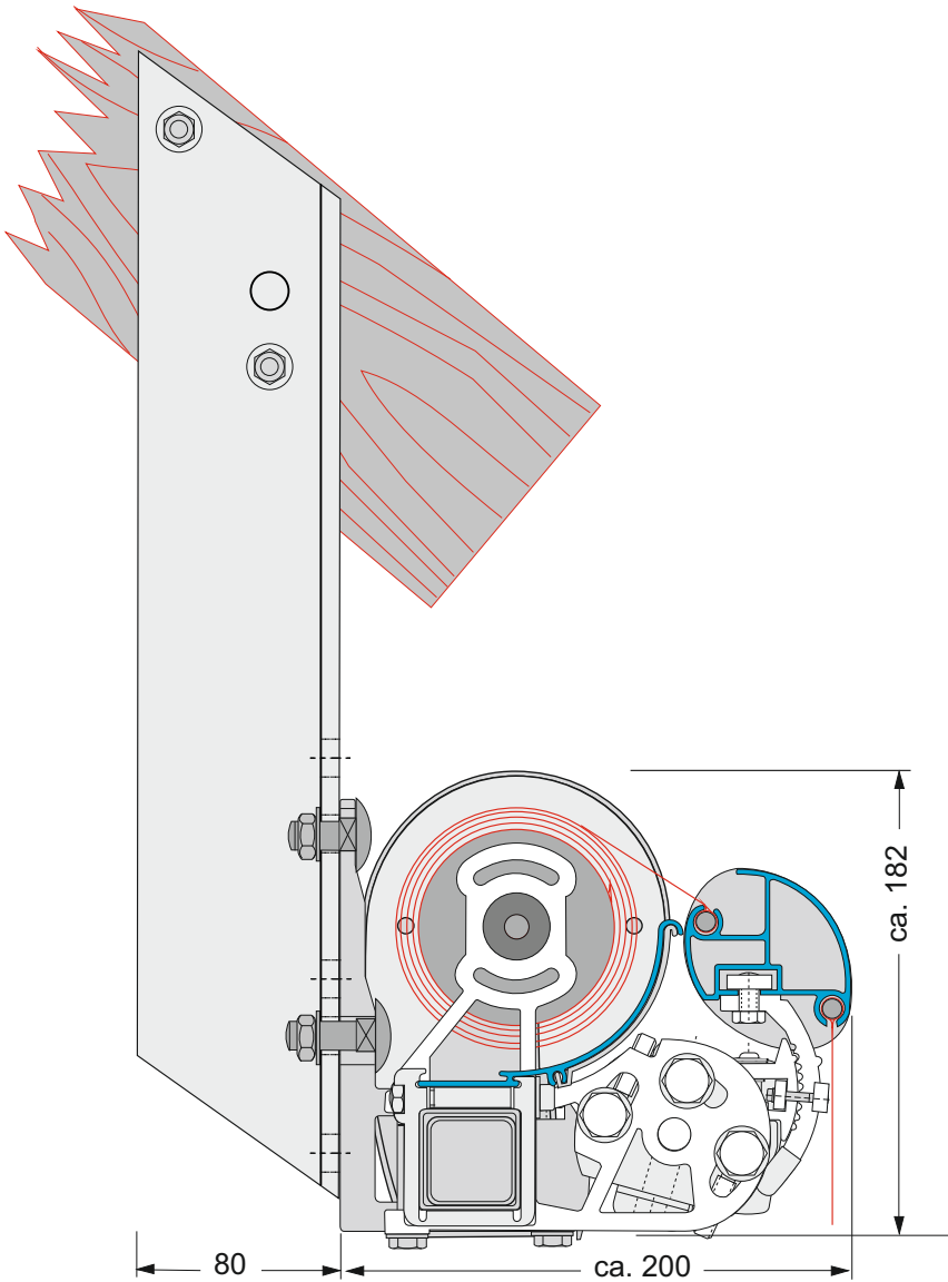
Dachsparrenmontage Rafter mounting
