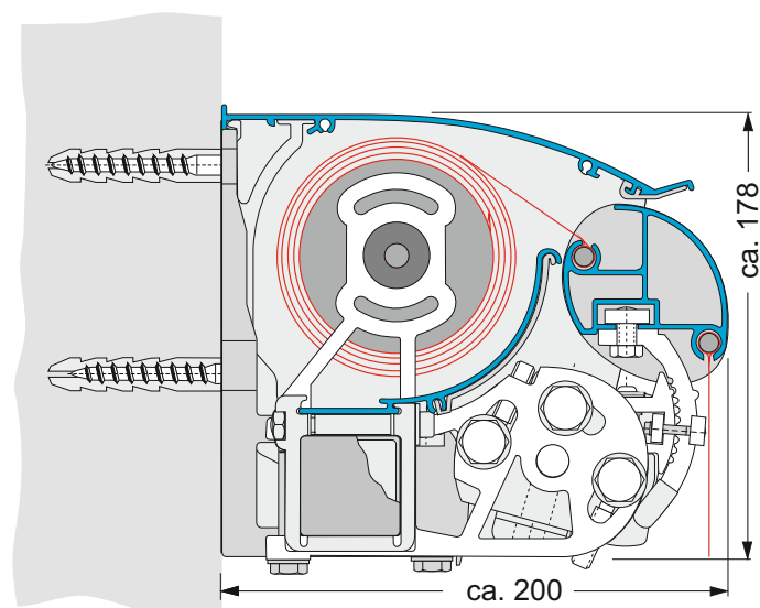
Wandmontage Wall mounting
