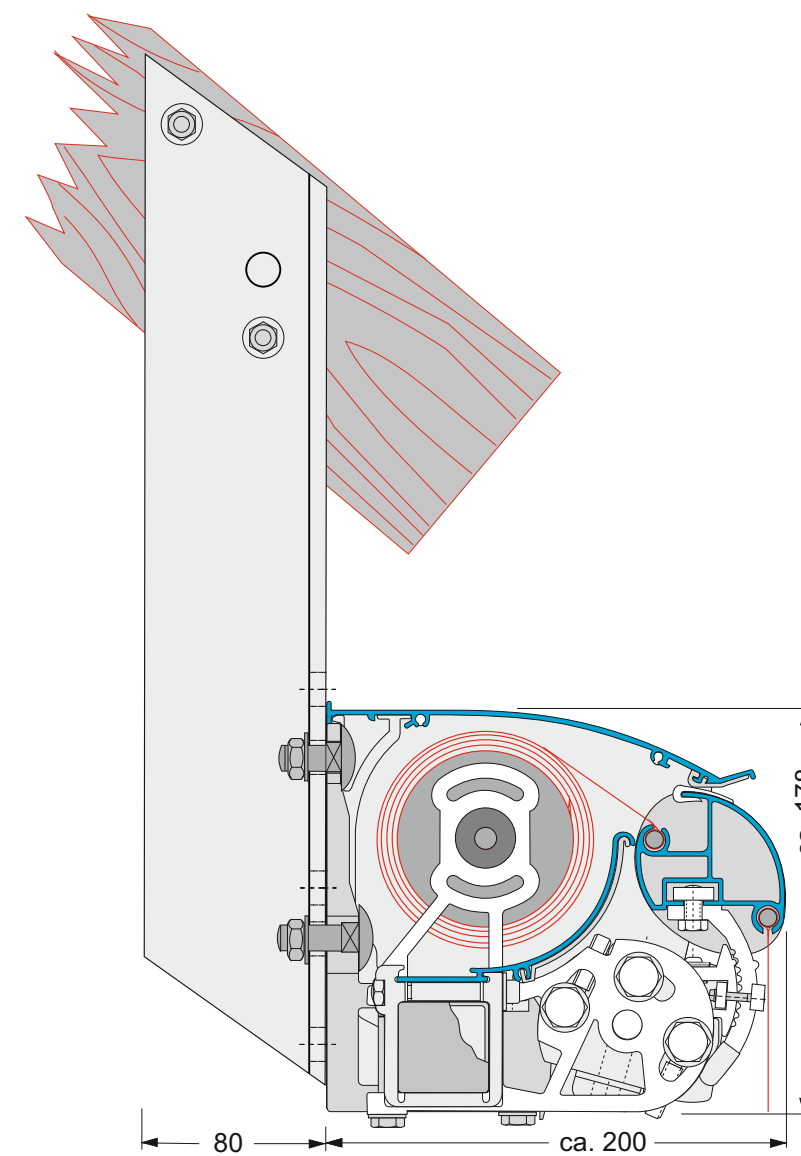
Dachsparrenmontage Rafter mounting
