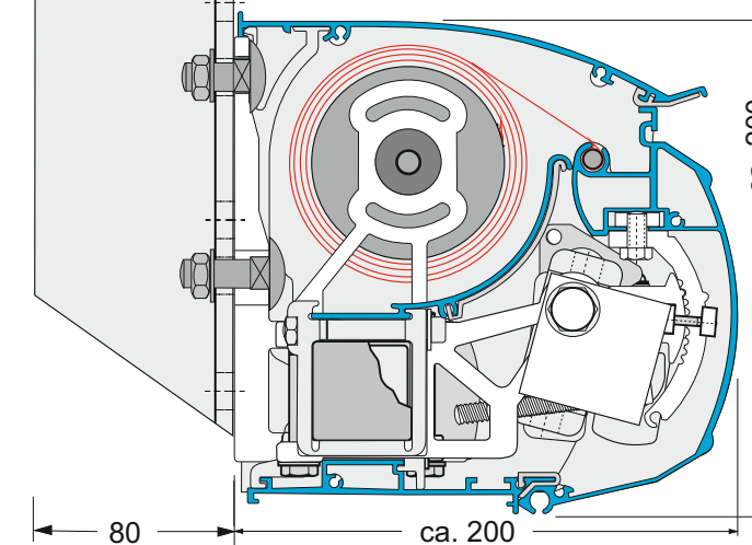
Dachsparrenmontage Rafter mounting
