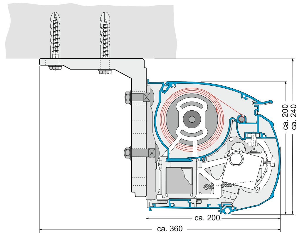
Deckenmontage Ceiling mounting
