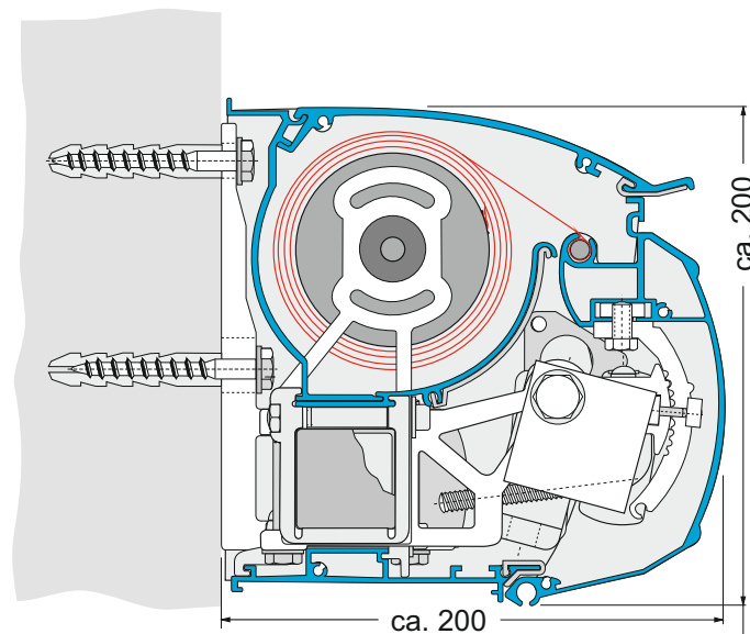
Wandmontage Wall mounting
