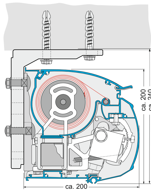
Deckenmontage Ceiling mounting
