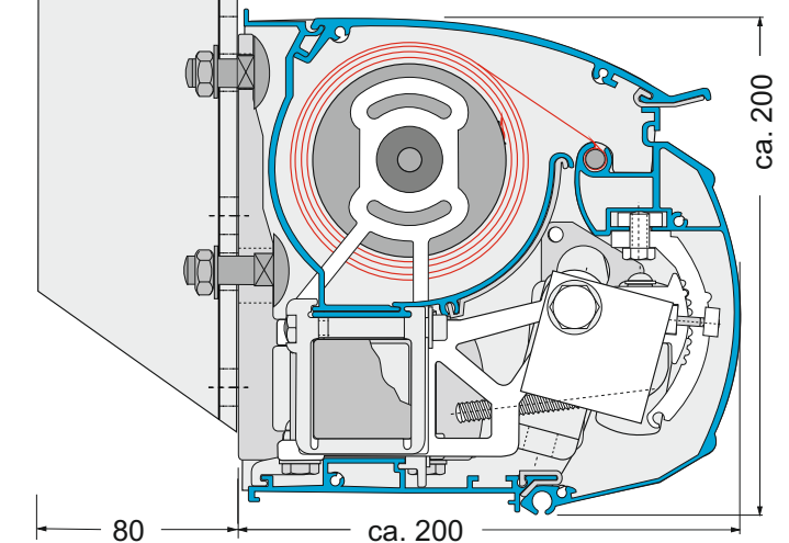
Dachsparrenmontage Rafter mounting
