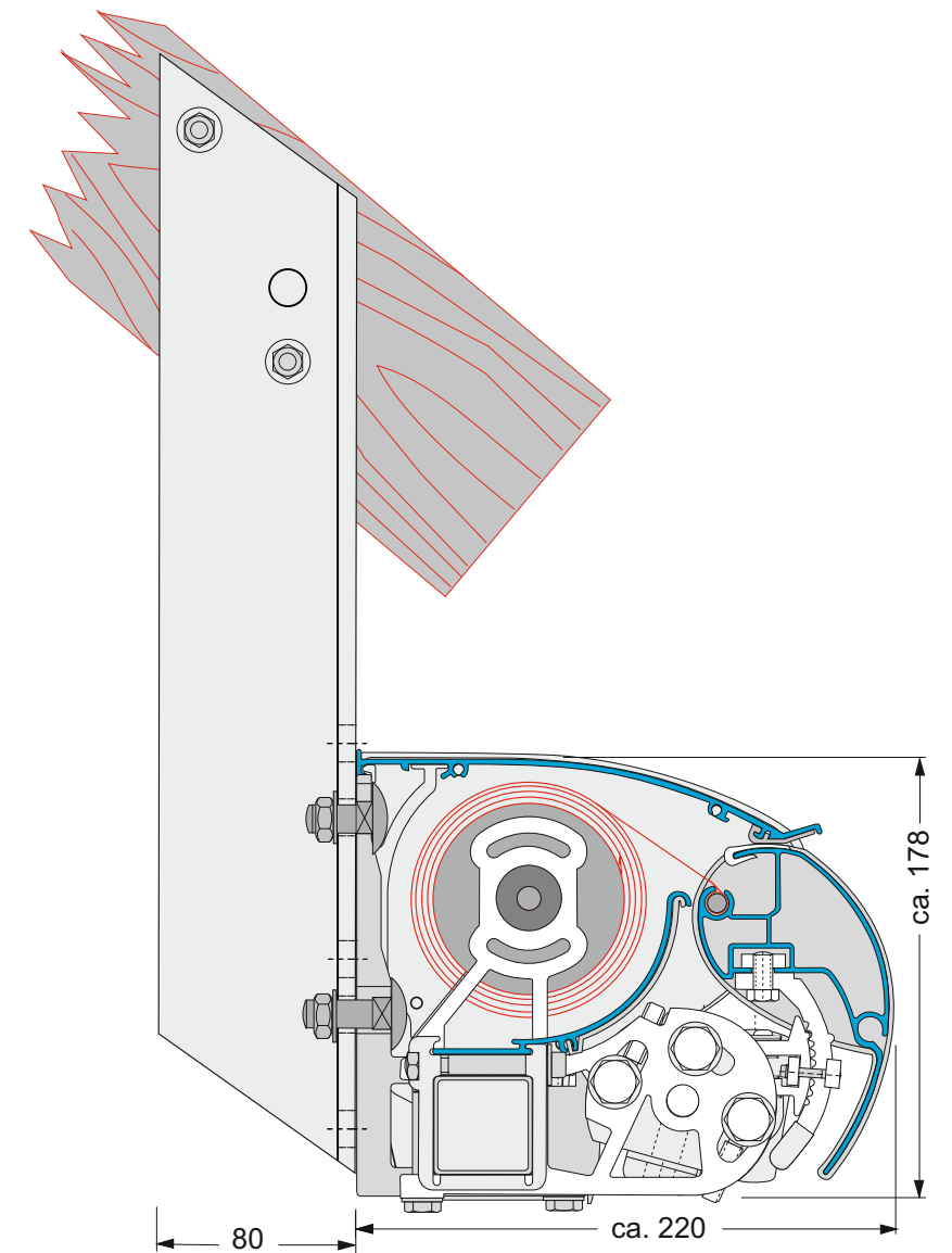
Dachsparrenmontage Rafter mounting
