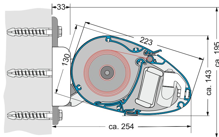
Wandmontage Wall mounting
