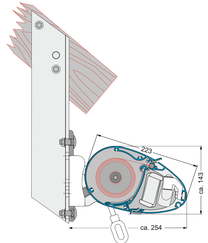
Dachsparrenmontage Rafter mounting
