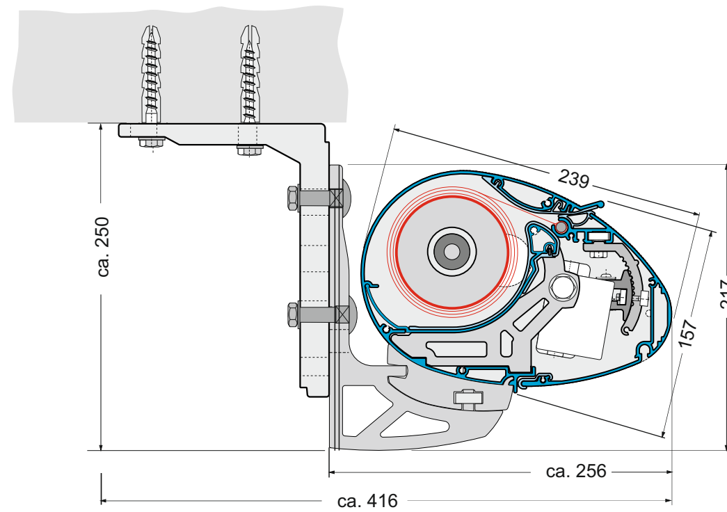
Deckenmontage Ceiling mounting
