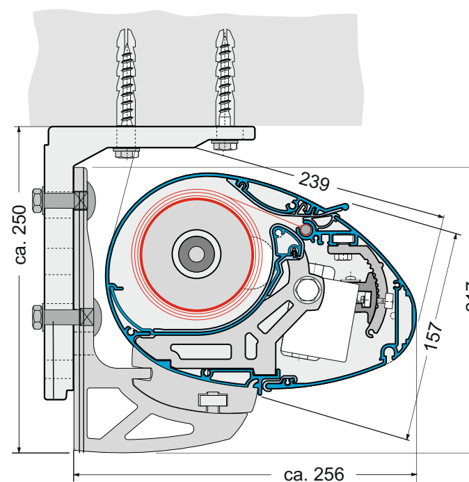
Deckenmontage Ceiling mounting
