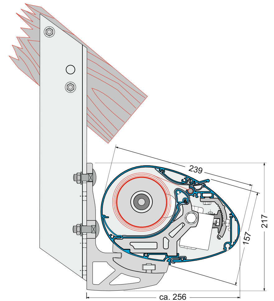
Dachsparrenmontage Rafter mounting
