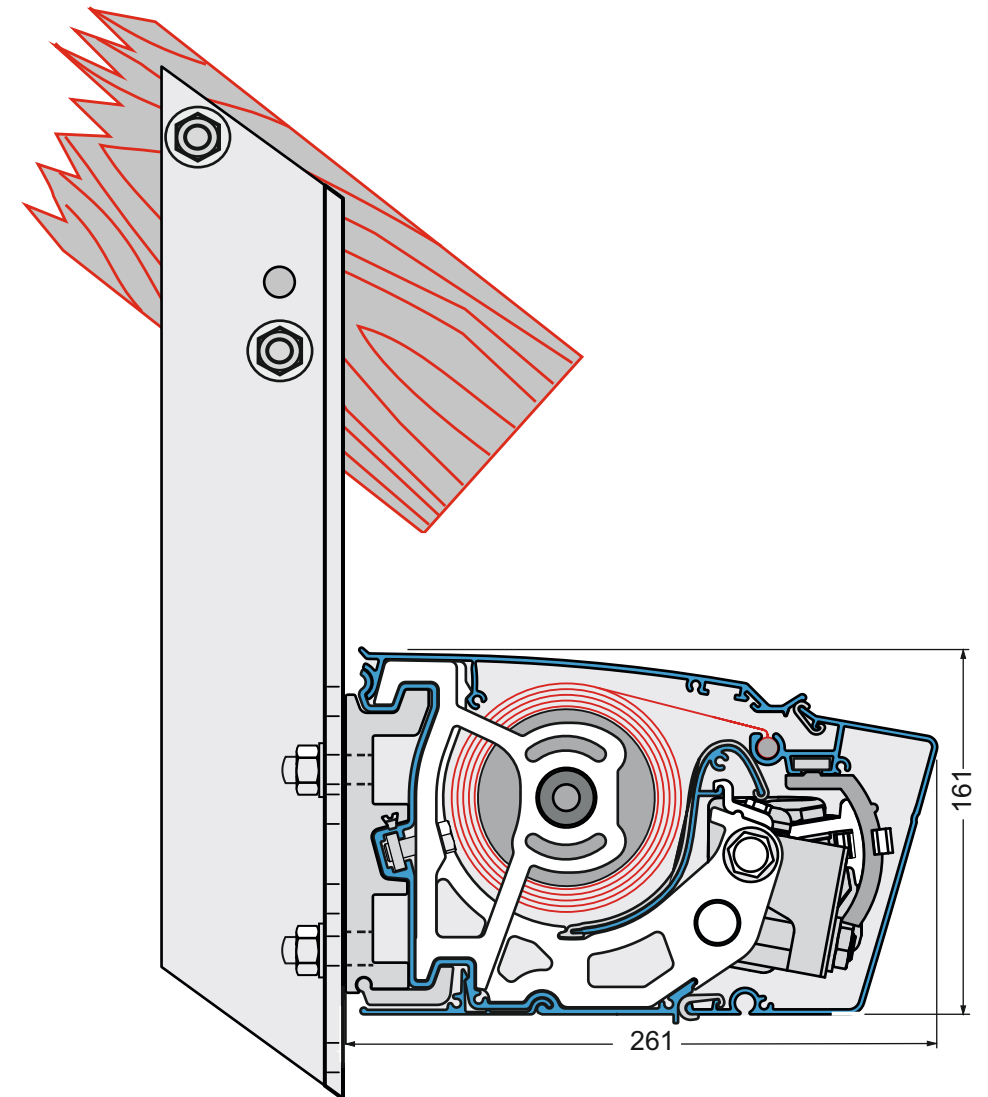
Dachsparrenmontage Rafter mounting
